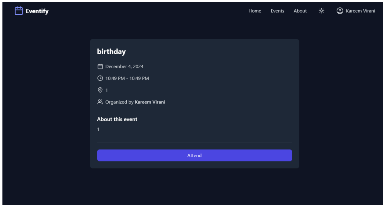
Event Details page
